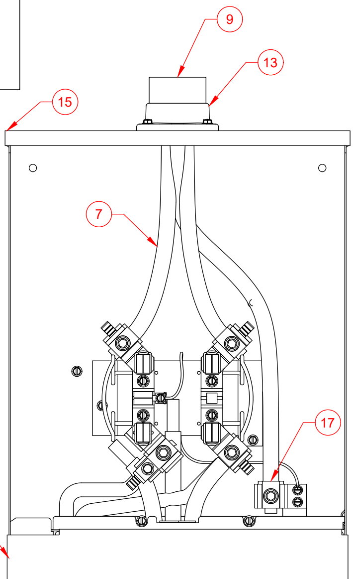
DETAIL A SCALE 1:4
