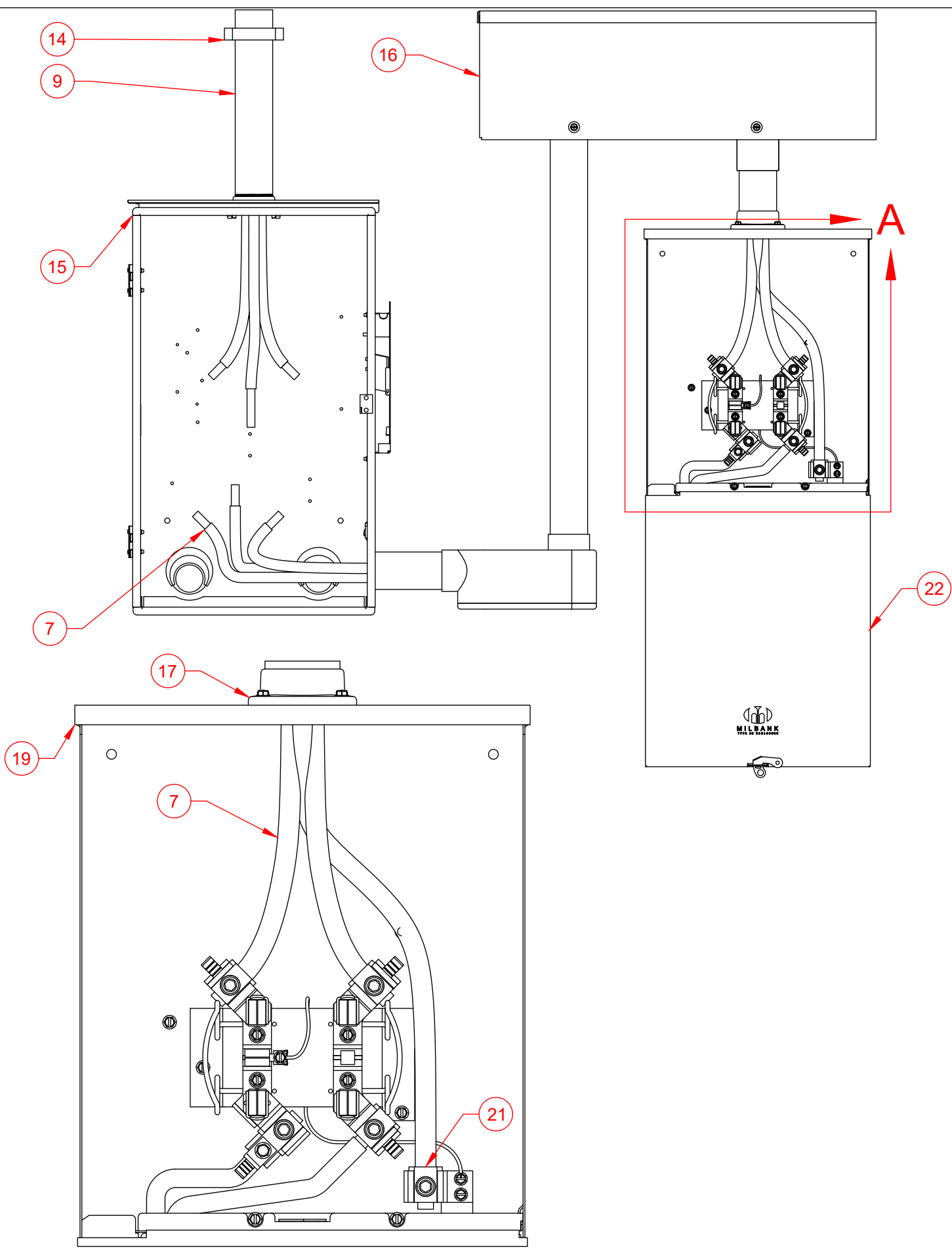
DETAIL A SCALE 1:4
