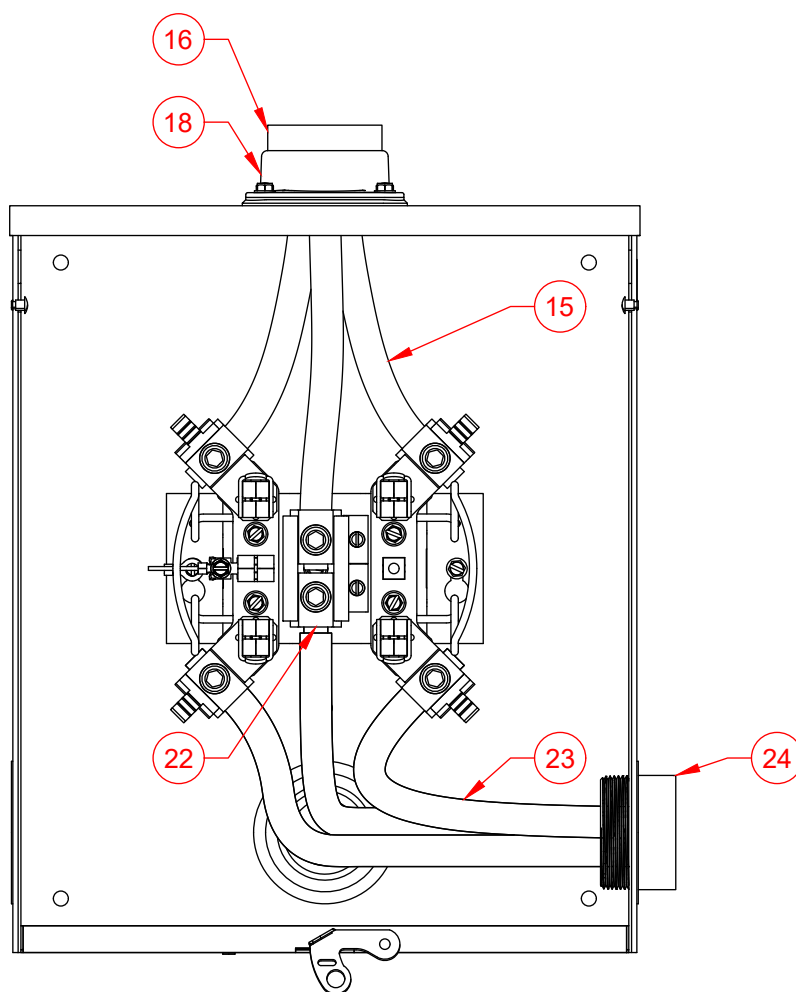
DETAIL B SCALE 1:4
